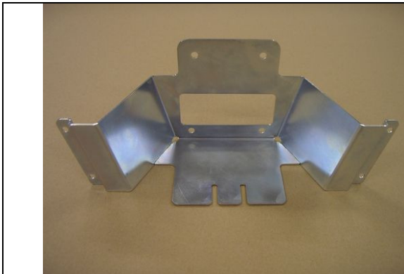
022.031.048 Front Stiffening Max Fire for Astro
