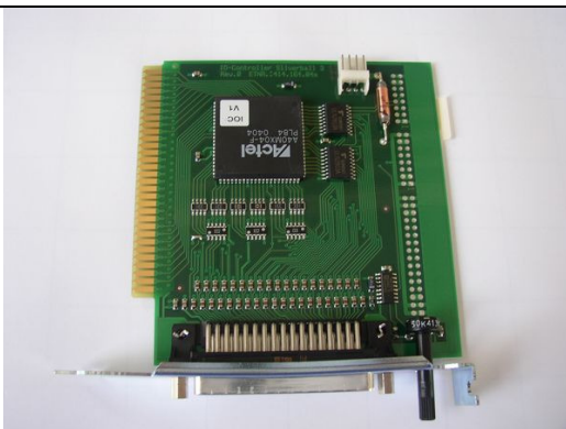
414.164.058 Platine I/O-Controller SB Pro
