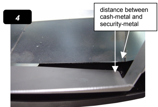
Before you mount the security-metal sidwise, Be careful, that there is enough distance between cash-metal and security-metal. Otherwise the cashbox don't match. Open and close the cash door to define the right distance.
