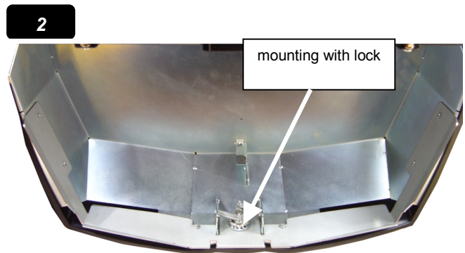
Dismount the locking mechanism and mount the security-metal under the lock.
