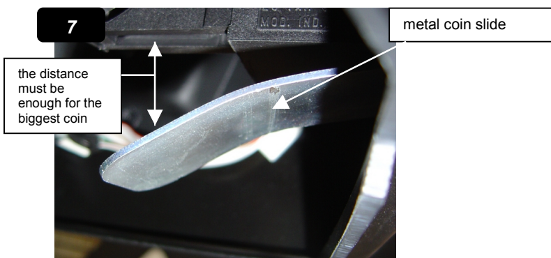
Form the coin-metal upward otherwise the coins get stuck.
